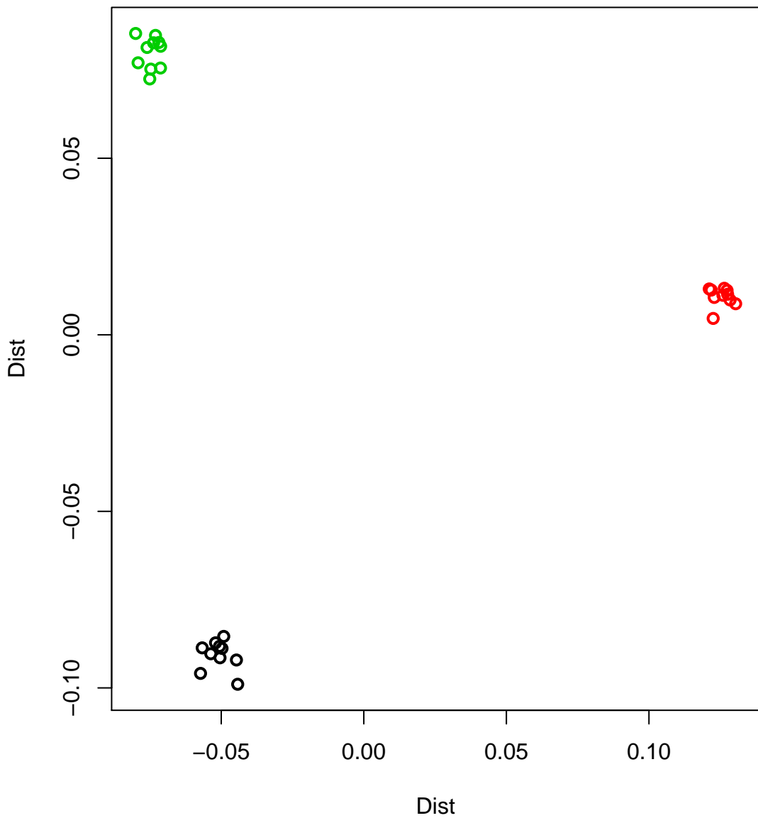
multidimensional scaling
