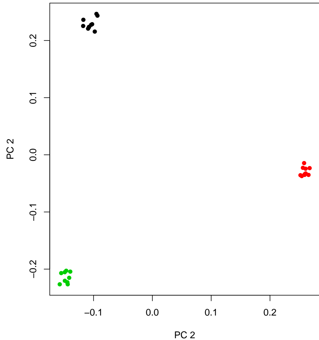
Principal components
